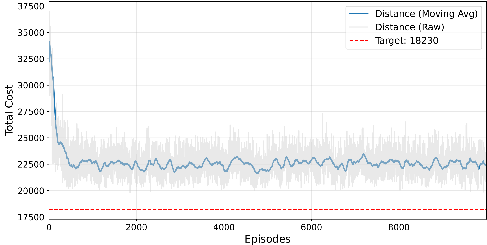
Final NO_BAYESIAN Masked AutoRL-SOP (HyperTuningSK) Training - ESC78.sop
